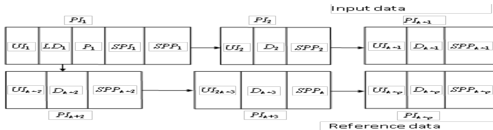
Figure2. Structure of the program of processing of databanks
